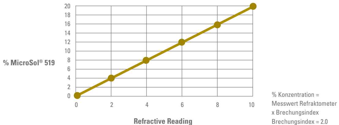
Concentration vs Refractive Index
